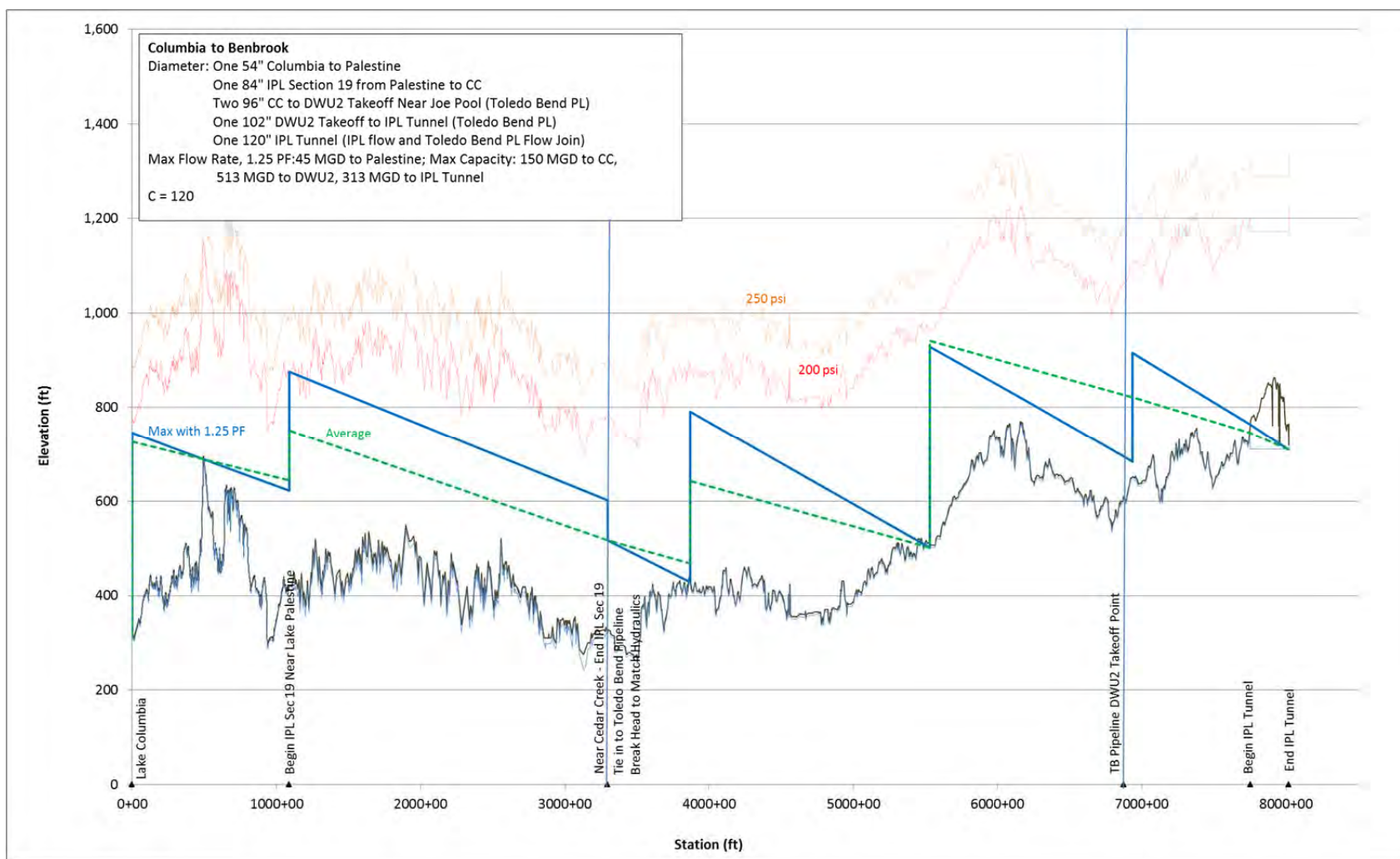
Hydraulic Grade Line - Lake Columbia to Lake Palestine
