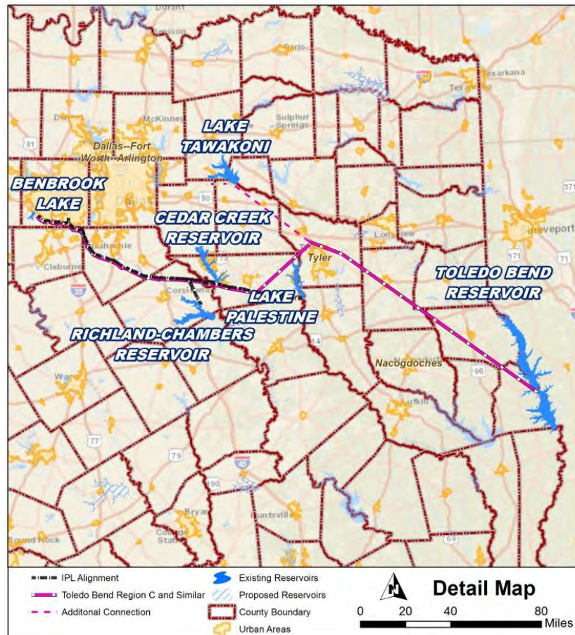
Figure 4.24 – Proposed Pipeline Route for Toledo Bend Reservoir
