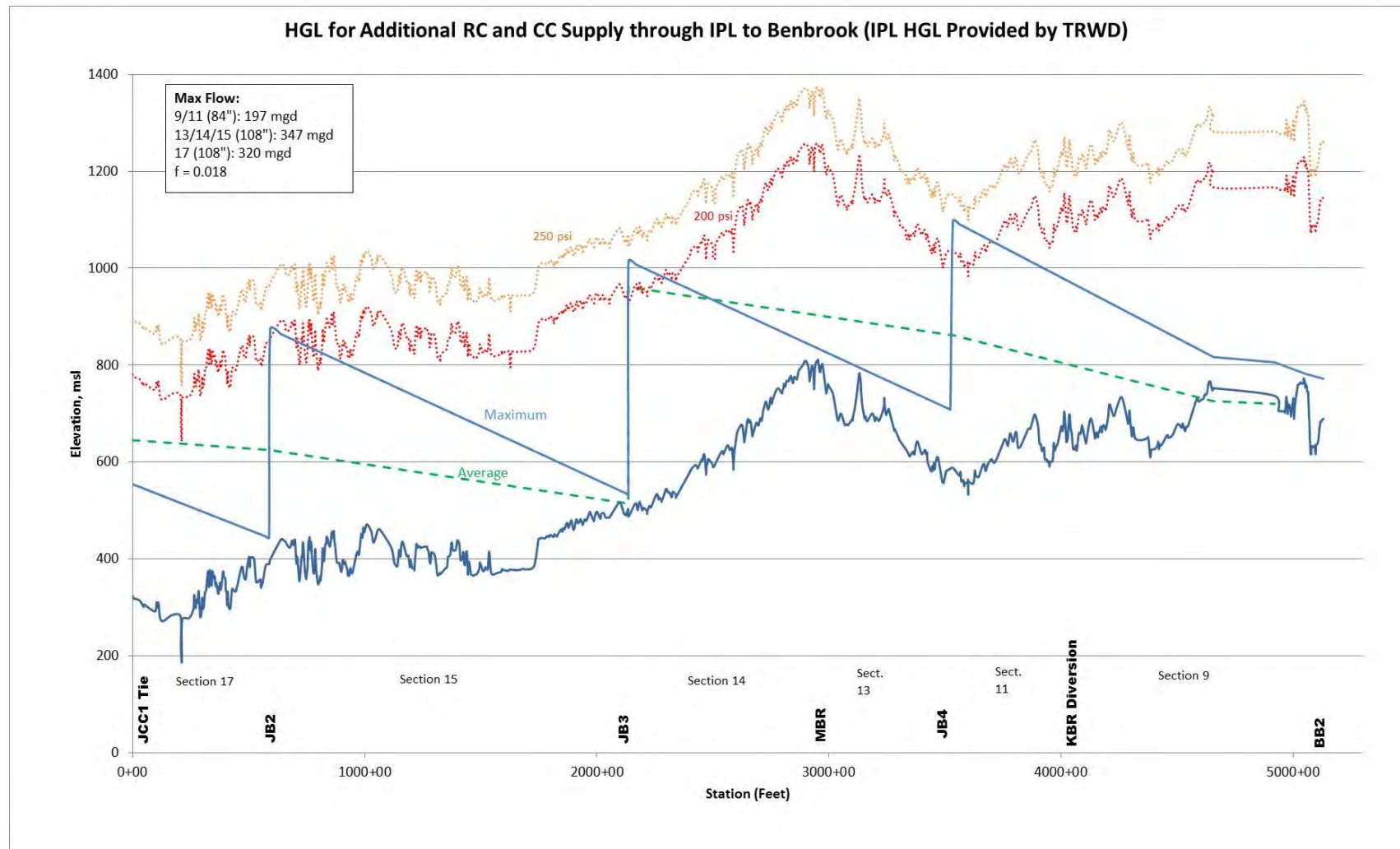
Hydraulic Grade Line –Richland Chambers and Cedar Creek Unpermitted Firm Yields through IPL
