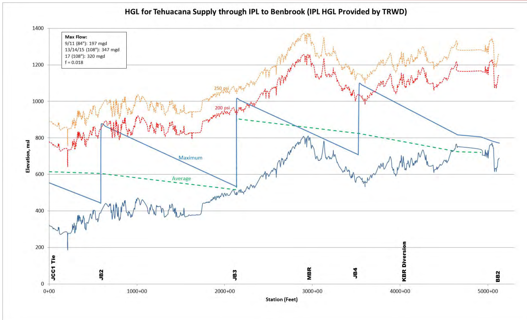
Hydraulic Grade Line – Tehuacana through the IPL to Lake Benbrook
