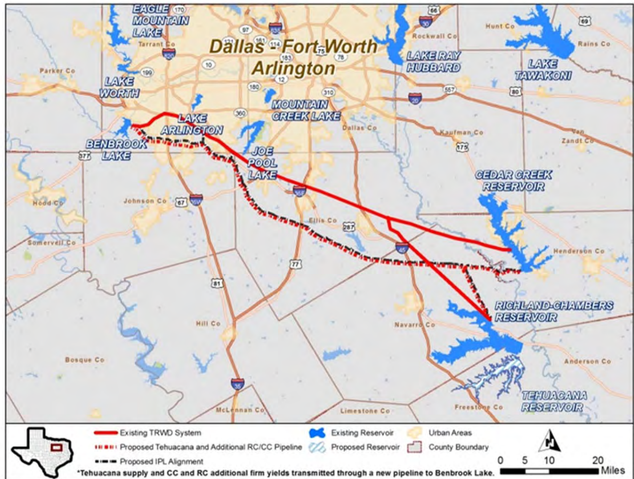
Pipeline Route to Lake Benbrook (Tehuacana and Additional Richland-Chambers & Cedar Creek in a new Pipeline Parallel to IPL)
