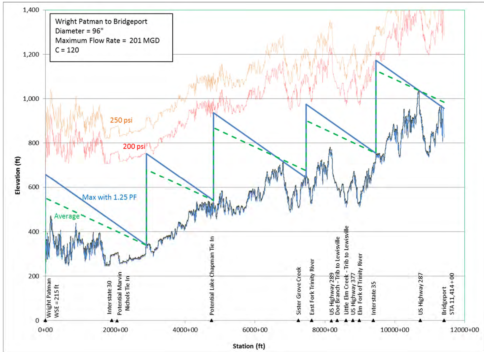
Hydraulic Grade Line – Lake Wright Patman to Lake Bridgeport
