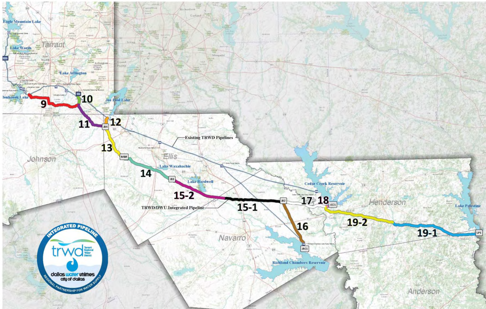
Figure 2.3 – Integrated Pipeline Project
