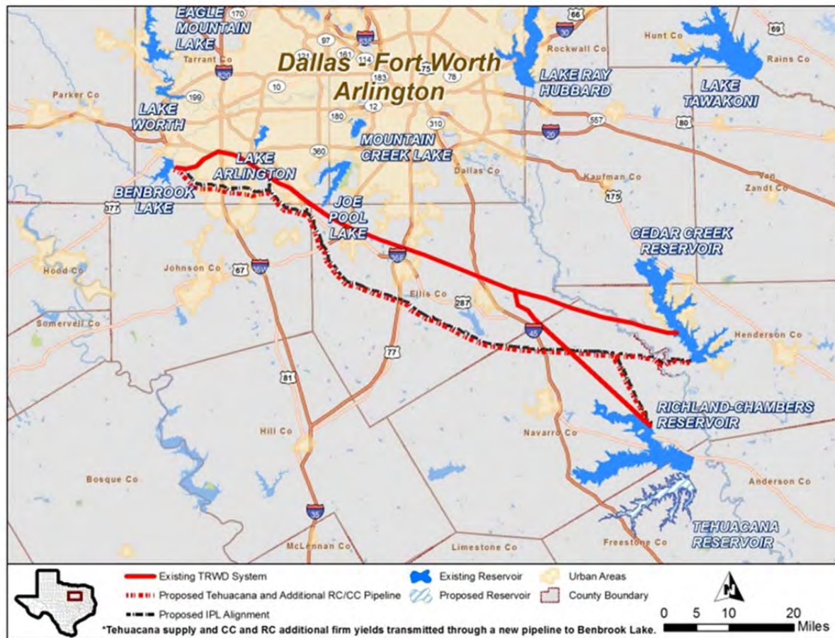
Pipeline Route to Lake Benbrook (Tehuacana Supply and Additional Richland-Chambers & Cedar Creek Unpermitted Supplies in a new Pipeline)
