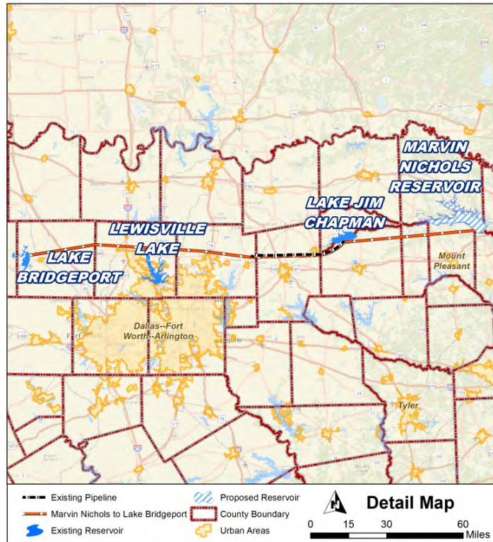
Pipeline Route Map
