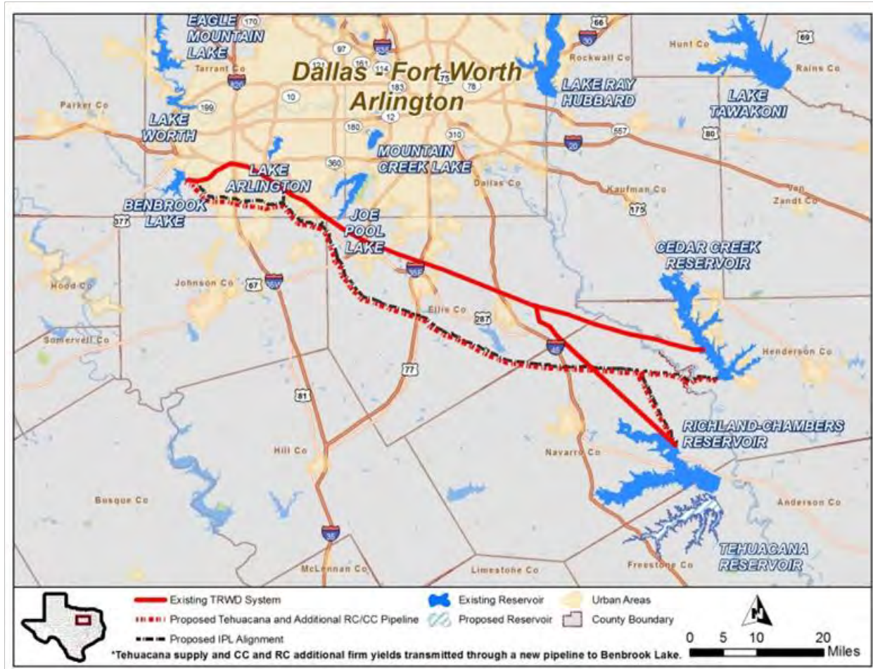
Figure 4.8 – Pipeline Route to Lake Benbrook (Tehuacana and Richland-Chambers & Cedar Creek Constructed Wetlands Supply in a New Pipeline Parallel to IPL)
