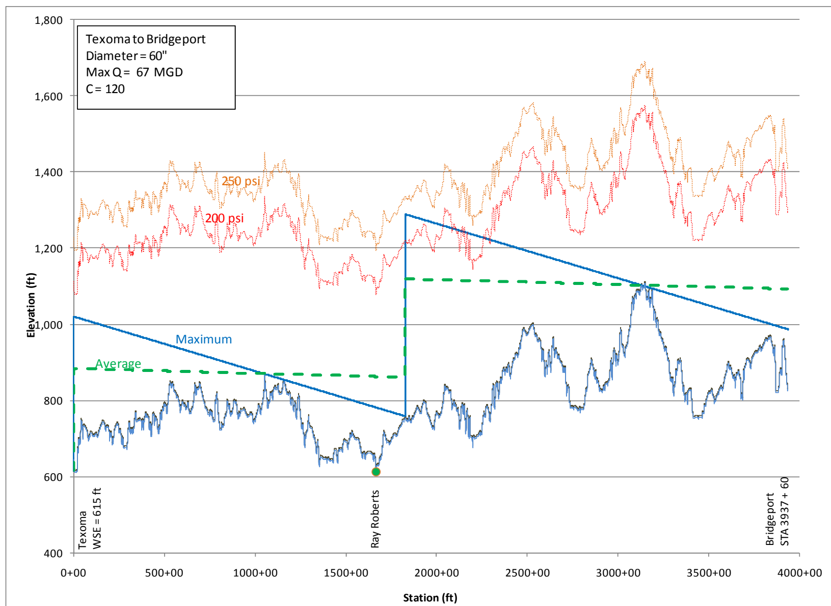
Hydraulic Grade Line - Lake Texoma to Lake Bridgeport
