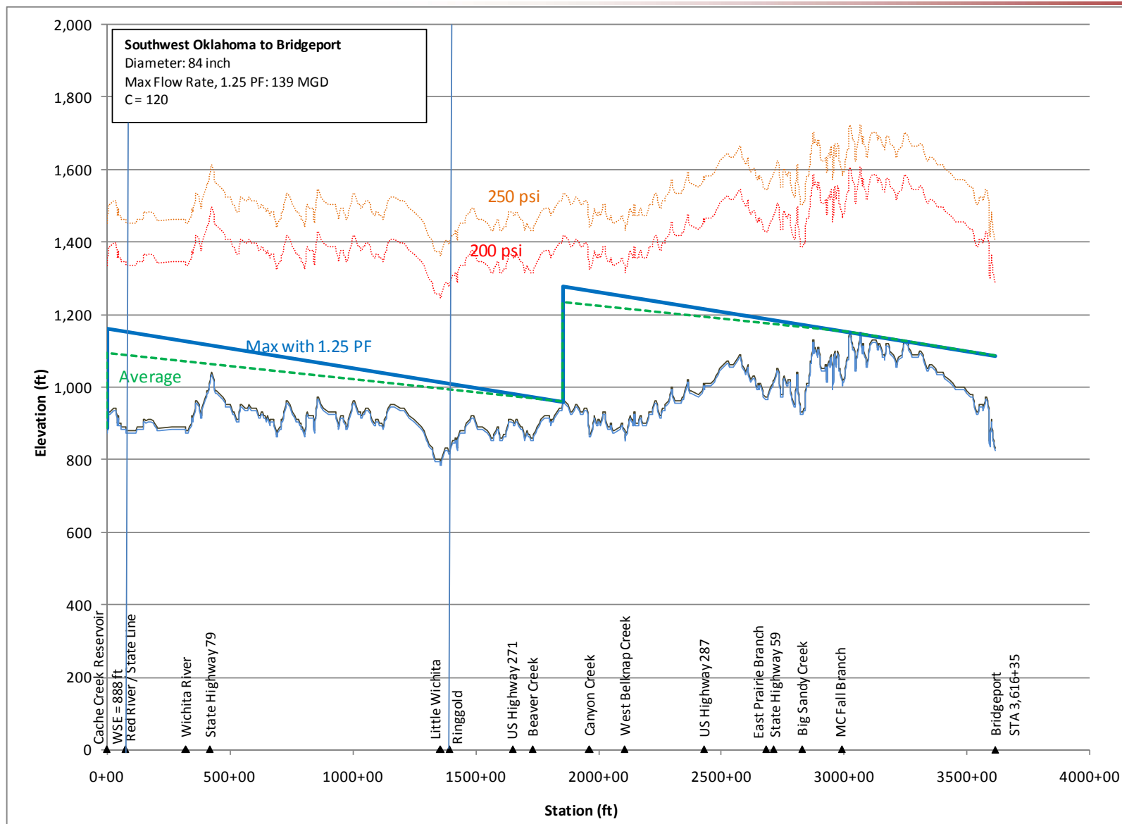
Hydraulic Grade Line - Temple Reservoir to Lake Bridgeport
