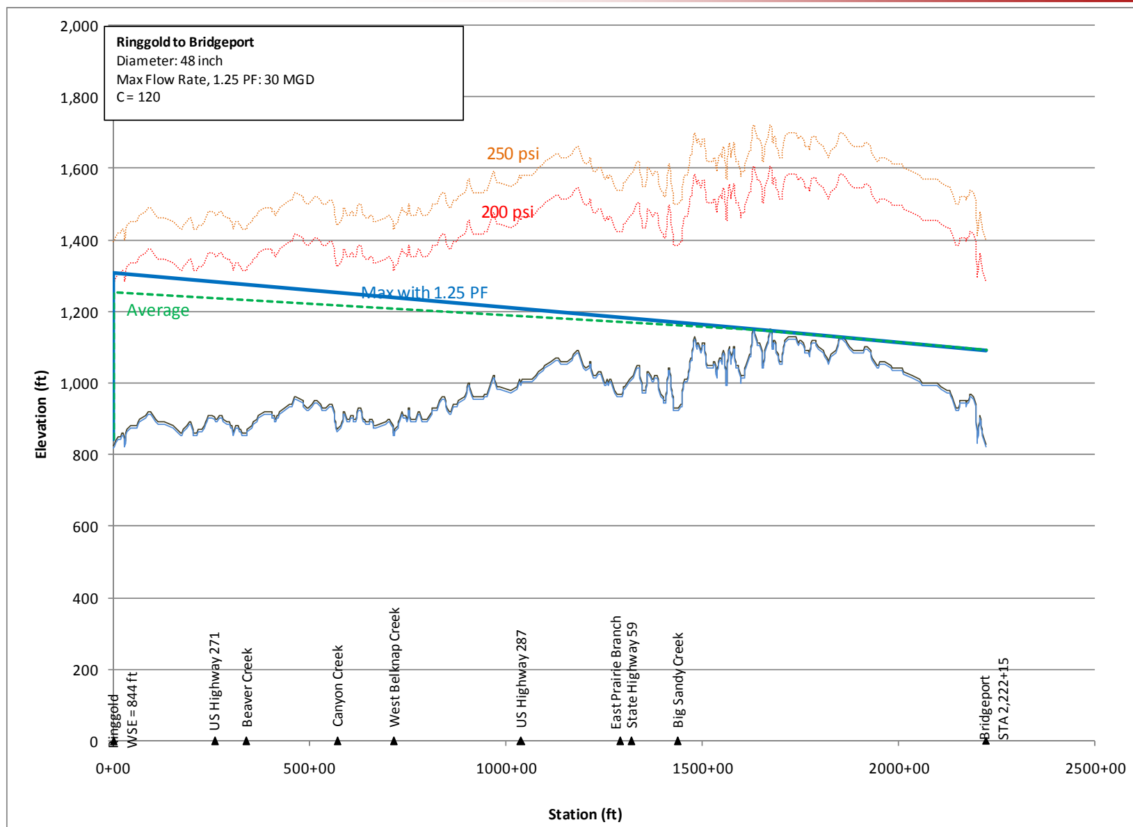
Hydraulic Grade Line – Lake Ringgold to Lake Bridgeport
