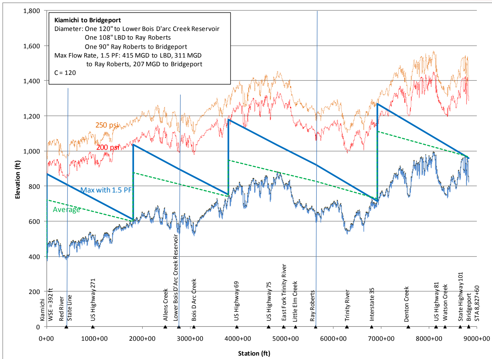
Hydraulic Grade Line - Kiamichi to Lake Bridgeport
