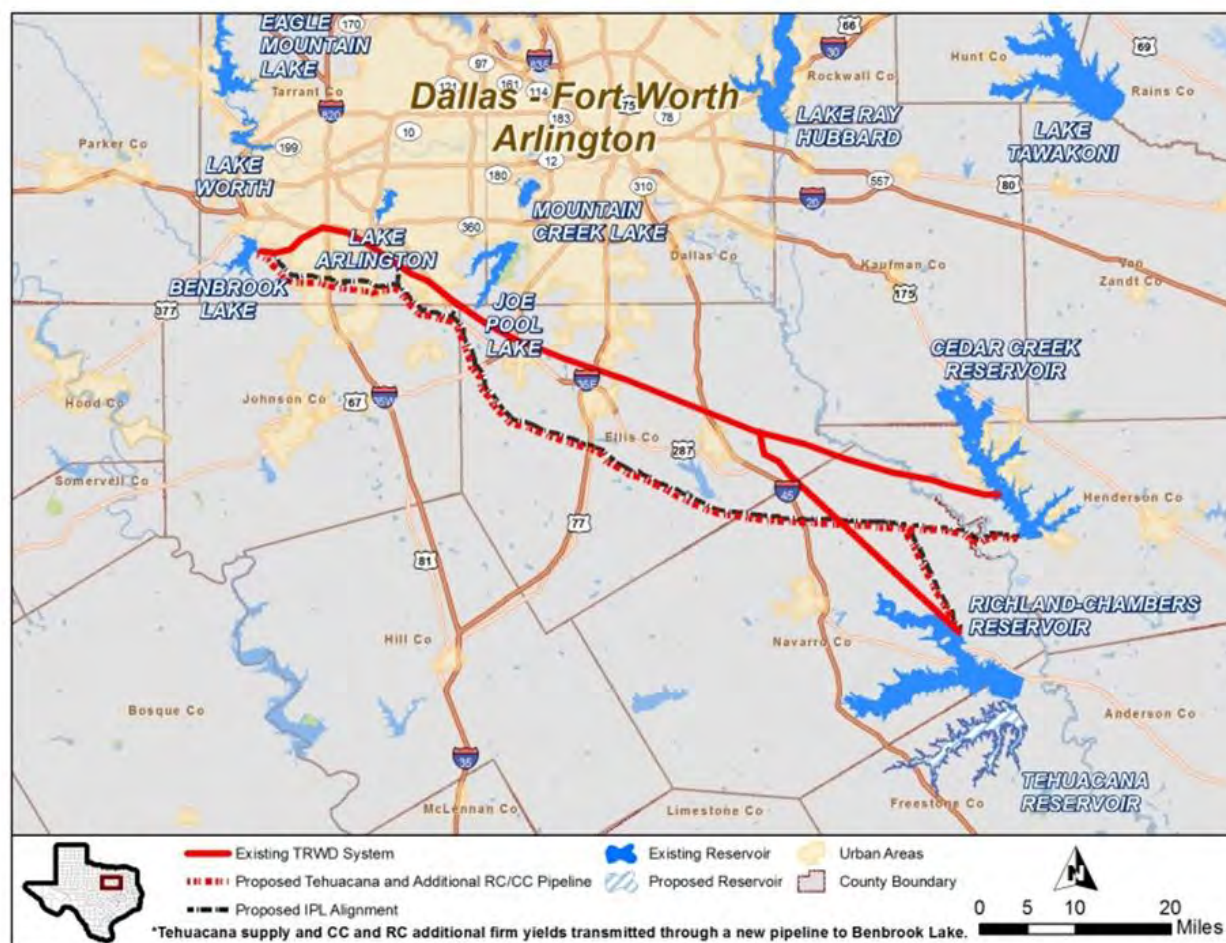
Figure 4.18 – Pipeline Route to Lake Benbrook (Tehuacana Supply and Additional Richland- Chambers & Cedar Creek Unpermitted Supplies in a new Pipeline)
