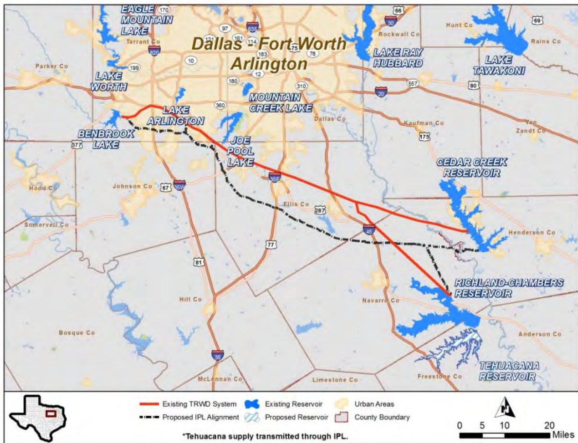
Pipeline Route to Lake Benbrook (Tehuacana supply transmitted through IPL)
