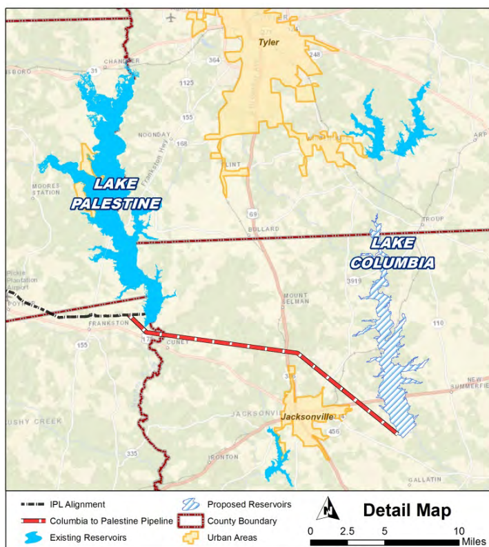
Pipeline Route to Lake Palestine
