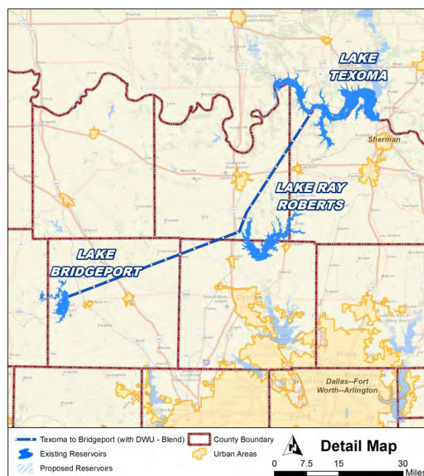
Pipeline Route Map
