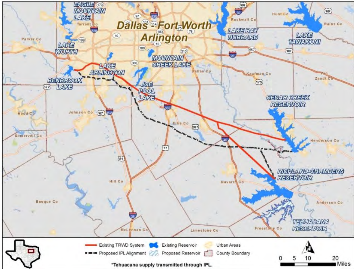
Figure 4.17 – Pipeline Route to Lake Benbrook (Tehuacana supply transmitted through IPL)
