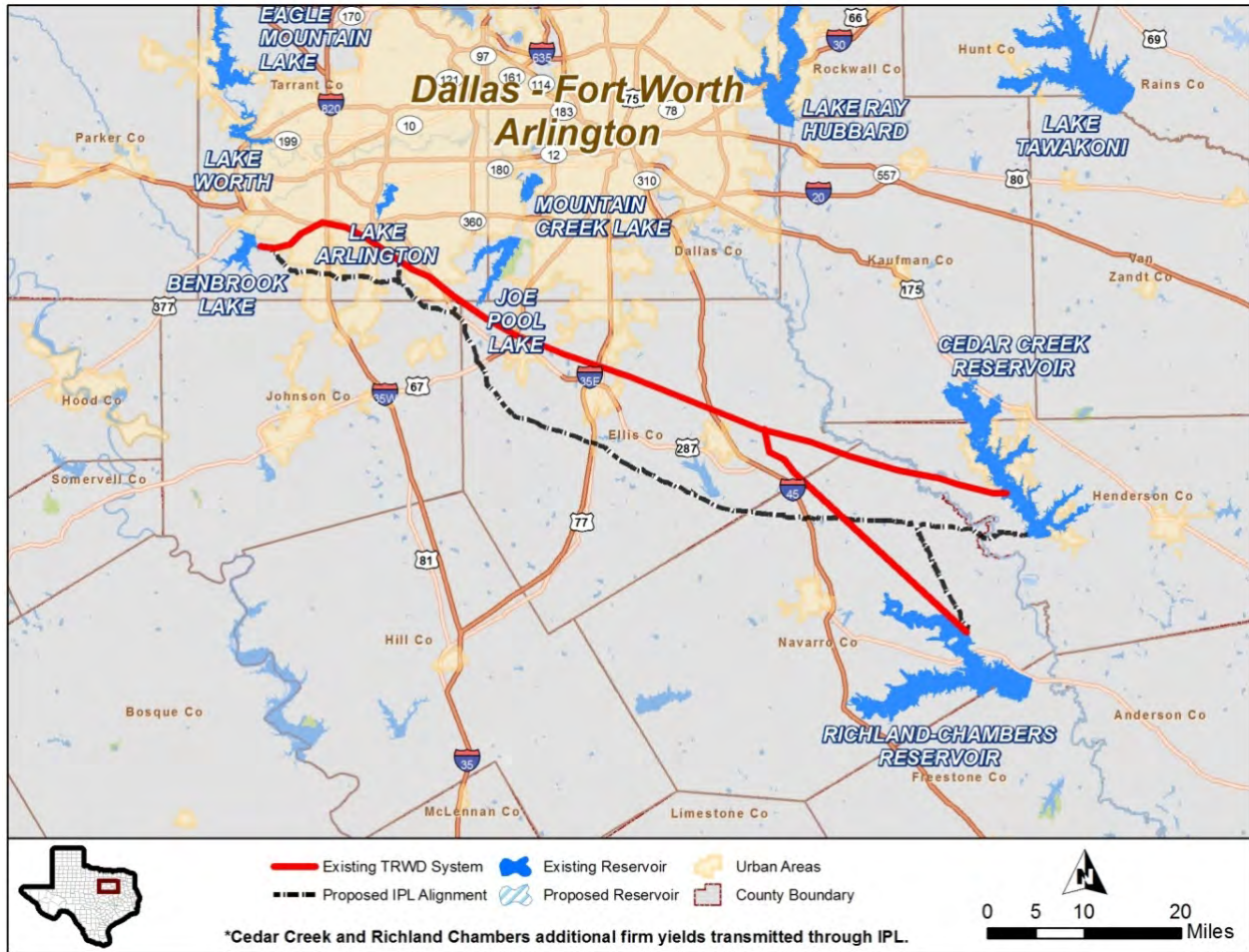
Pipeline Route to Lake Benbrook (Transmitted through IPL)
