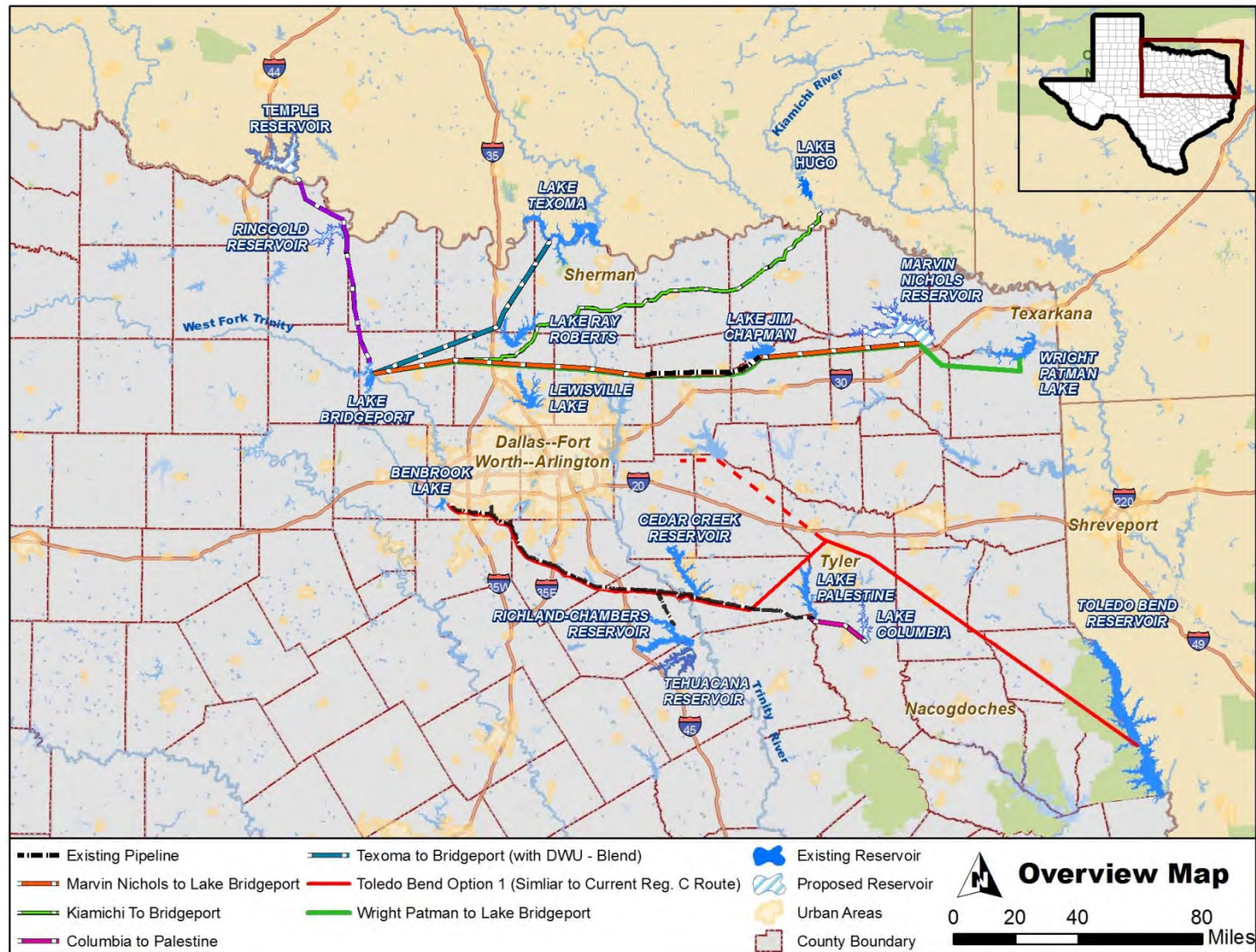
Figure ES.3 – Water Management Strategies’ Transmission Routes
